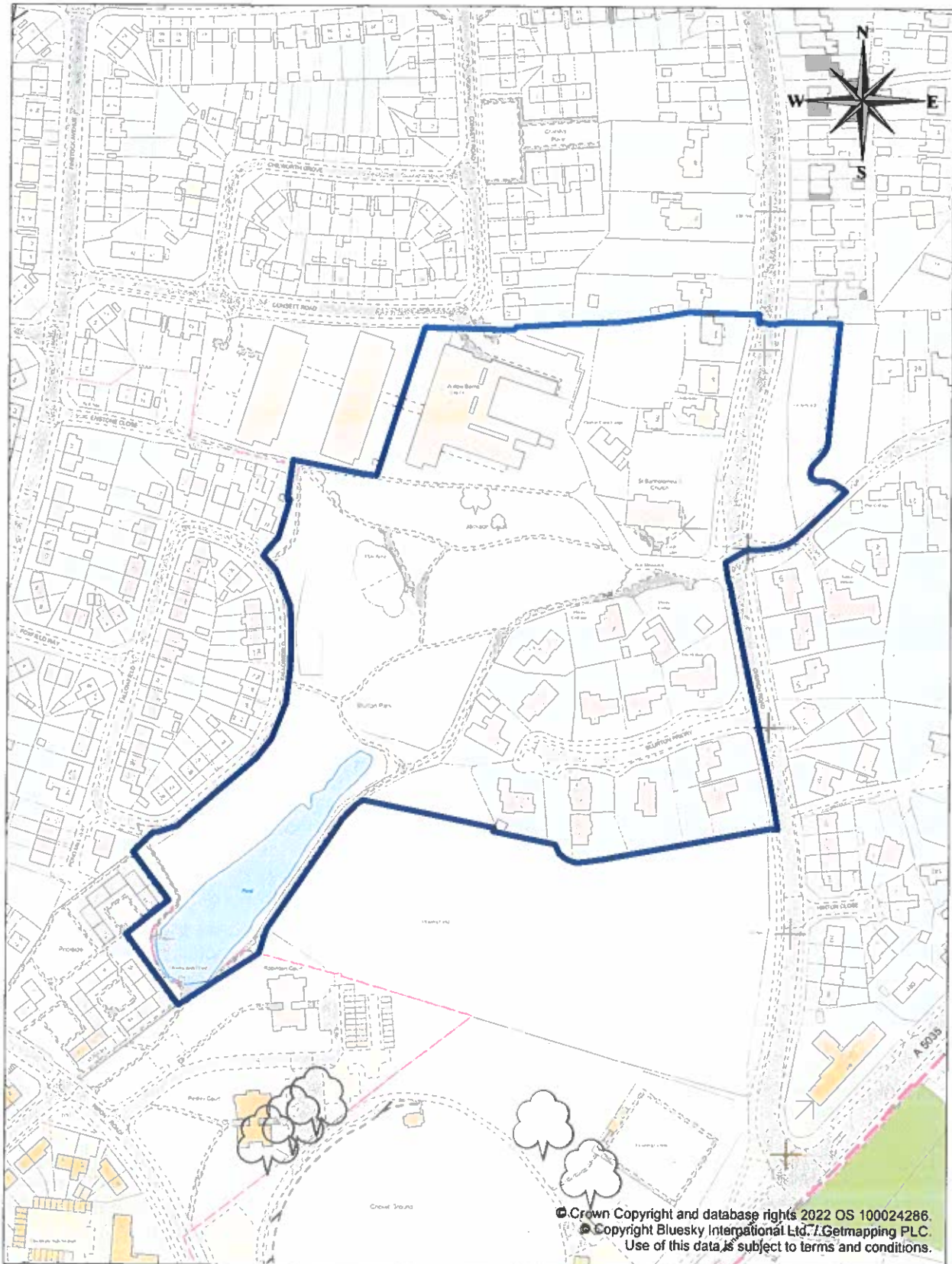
Map B: Blurton Church Conservation Area - Proposed
